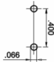
MOUNTING HOLE DIAGRAM
